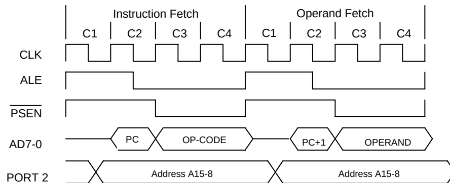
Figure 4. Two Cycle Instruction Timing
